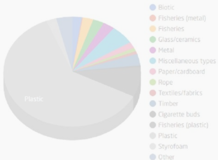
Global composition of marine litter
